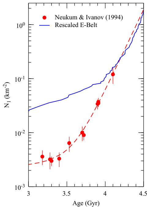
Fig. 2. The dash-red curve is the total number of craters larger than 1 km diameter per km 2 as a function of unit's age, according to NI94. The blue curve is the same, but here we assumed (i) the E-belt model, (ii) the E-belt was destabilized 4.5 Gy ago and (iii) the E-belt contained 20 times more material than used by Bottke et al. (2012). This allowed us to match the extrapolation of the NI94 curve at 4.5 Gy. Notice the overall mismatch for ages younger than 4 Gy ago. (For interpretation of the references to color in this figure legend, the reader is referred to the web version of this article.)
