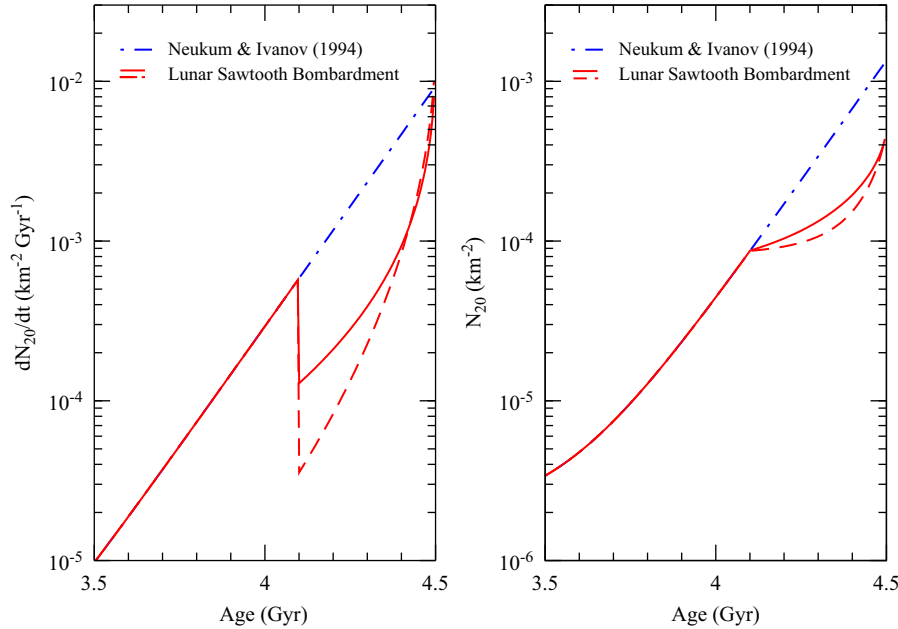
Fig. 3. The timeline of lunar bombardment. The blue dash-dotted line is the exponential decay assumed by NI94. The red curves show our results combining a post-accretion bombardment of leftover planetesimals in the 4.1–4.5 Gy time range and the asteroid main belt and E-belt bombardments for t < 4.1 Gy. The solid and dashed curves for t > 4.1 Gy correspond to the two analytic functions that bracket the early decay of the cratering rate, as discussed in the text. The left panel shows the bombardment rate as a function of time (measured in number of craters larger than 20 km produced per km 2 and per Gy). The right panel shows the cumulative bombardment suffered by a given terrain as a function of its age (measured in number of craters larger than 20 km per km 2 , i.e., N_{20} ). On the left panel, the equations of for the curves are the following. For t < 4.1 Gy: dN_{20}/dt = 2.7 \times 10^{-16} e^{6.93t} + 5.9 \times 10^{-7} ; for t > 4.1 Gy and the solid curve: dN_{20}/dt = 2.5 \times 10^{-2} e^{-((4.5-t)/0.003)^{0.34}} ; for the red dashed curve: dN_{20}/dt = 2.0 \times 10^{-2} e^{-((4.5-t)/0.01)^{0.5}} ; the time t is measured in Gy. (For interpretation of the references to color in this figure legend, the reader is referred to the web version of this article.)
