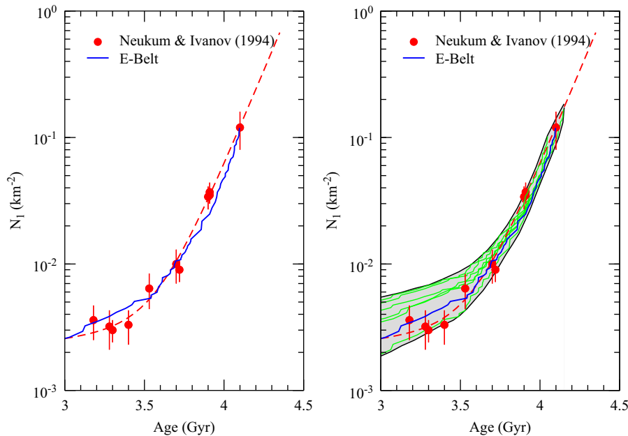
Fig. 1. In both panels, the dashed red curve shows the density of craters larger than 1 km diameter ( N_1 ) as a function of the unit's age, according to NI94. This curve has equation N_1 = 5.44 \times 10^{-14}(e^{6.93t} - 1) + 8.38 \times 10^{-4} t , where t is measured in Gy. The blue curve is the same, but it follows the E-belt model (Bottke et al., 2012), assuming that the E-belt was destabilized 4.1 Gy ago. The dots with the vertical error bars show the density of craters on the terrain calibration units according to crater counts and ages reported in NI94. The Nectaris basin data-point is the first from the right. Notice that the density of D > 1 km craters is not directly measured on the oldest units (because of saturation and degradation of small old craters and the presence of secondary younger craters); instead, it is estimated from the density of larger craters (typically with D > 20 km, i.e., N_{20} ) assuming a SFD for the crater production function. Here, for comparative purposes, for the E-belt model we have converted N_{20} into N_1 using the same crater SFD adopted in NI94. The green curves on the right panel show different E-belt models obtained by changing assumptions on the age of Orientale basin and on the total E-belt population within ranges that allow to fit the data reasonably well for t > 3.5 Gy. We also add the contribution of MB-NEAs, assuming different bombardment rates, constant with time and up to the current value. The shaded area is the envelope of the models that we consider acceptable. (For interpretation of the references to color in this figure legend, the reader is referred to the web version of this article.)
