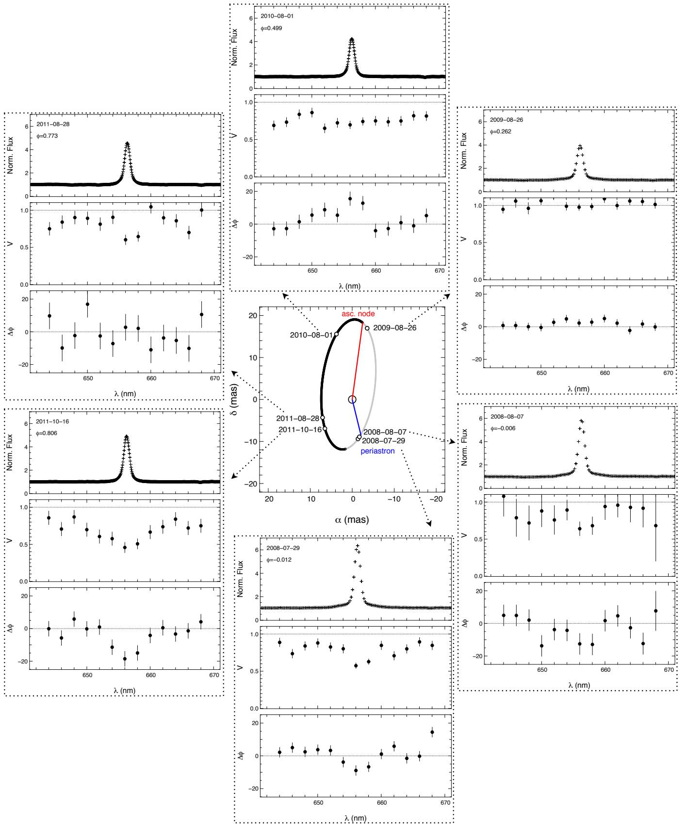
Fig. 4. VEGA spectro-interferometric measurements over the orbit.
