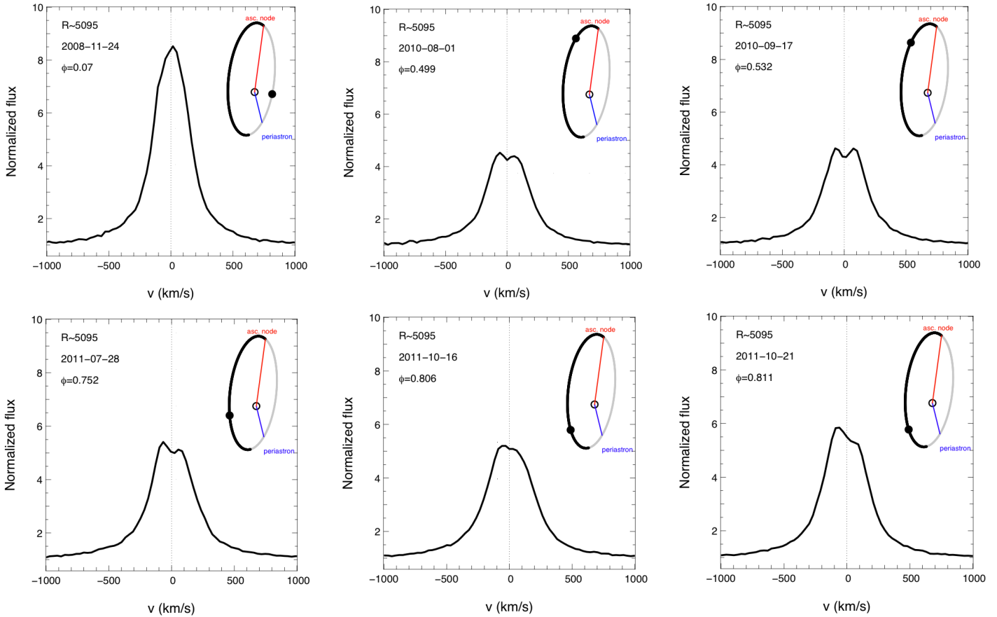
Fig. 3. Variation of the line profile measured with VEGA at R~5000, with the orbital phase. In each panel, the astrometric orbit is shown, with a full black circle indicating the corresponding orbital phase. The thick part is oriented towards the observer.
