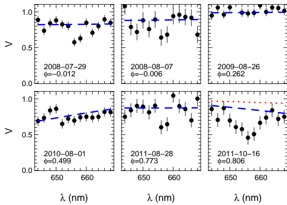
Fig. A.1. Best-fit binary models in the continuum (dashed blue line). The red dotted line in the lower right panel is the prediction of a binary model with flux ratio of FR=0.10 to which the continuum visibilities measured for \phi=0.806 were re-scaled.
