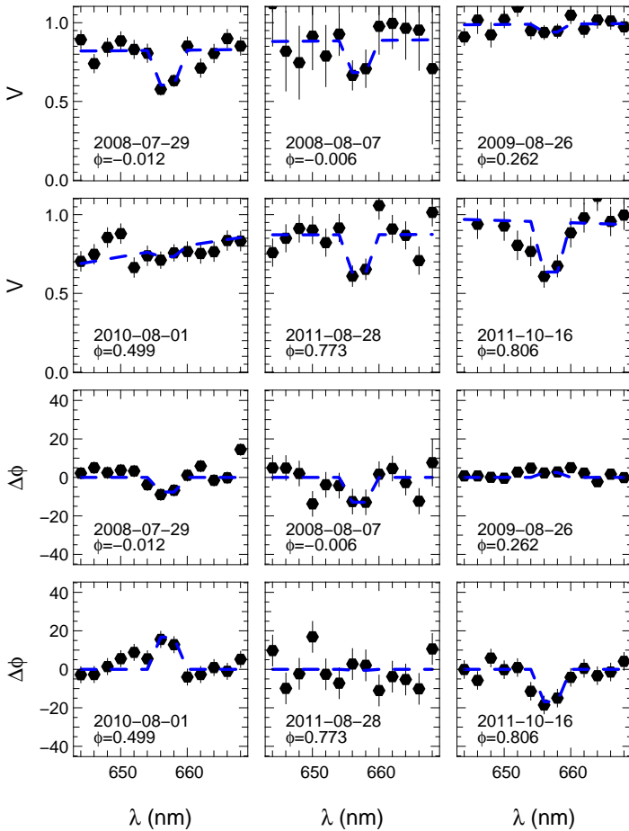
Fig. 5. Best-fit continuum and H \alpha line model (dashed line). The first two lines give the visibilities, the following two, the differential phases. We recall that the visibilities for \phi=0.806 have been scaled to the binary model with FR=0.10.
