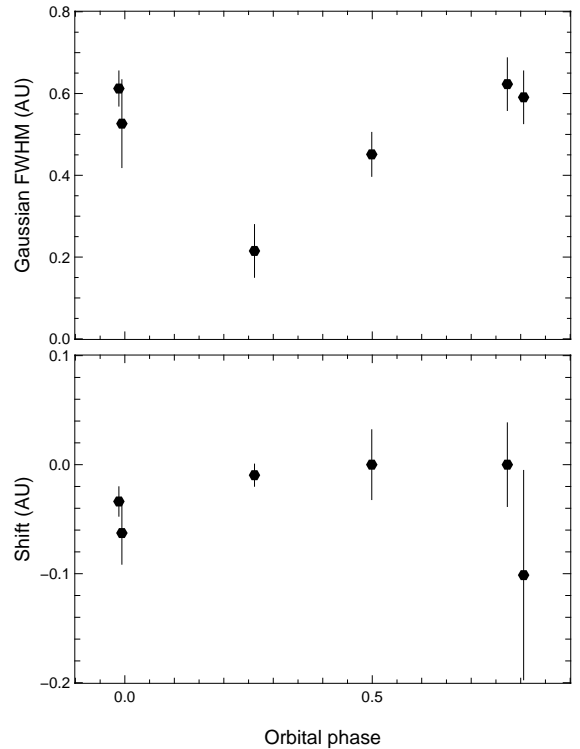
Fig. 6. Best-fit model parameters, Gaussian FWHM (top) and displacement (bottom), over the orbit.
