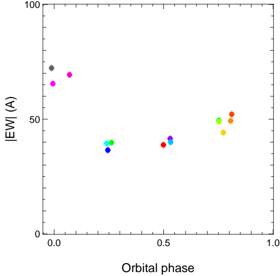
Fig. 2. Equivalent widths of the H_\alpha line over the orbit for all the spectra.
