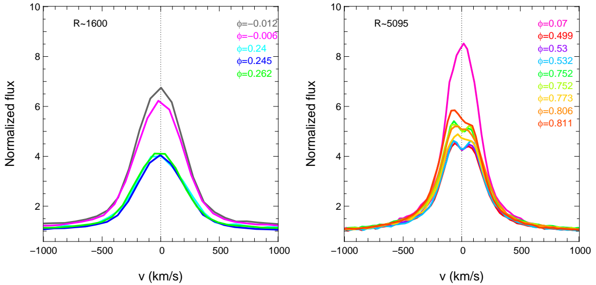
Fig. 1. Left: H \alpha VEGA spectra obtained at R=1600 (LR). Right: Additional VEGA spectra obtained at R=5000 (MR).
